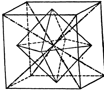
Axes of Trigonal Symmetry (Octahedral Axes)
